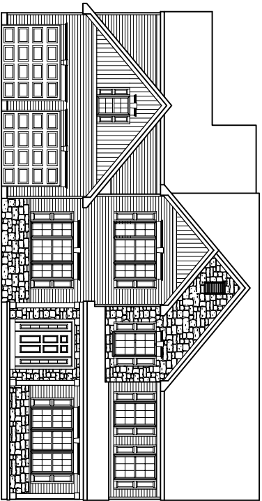
FRONT ELEVATION
