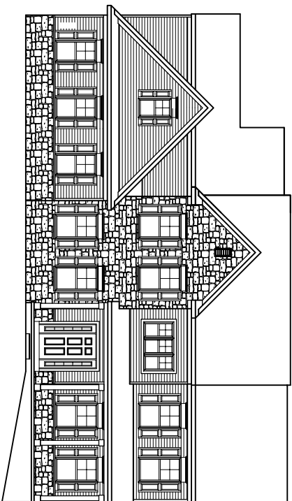
FRONT ELEVATION
