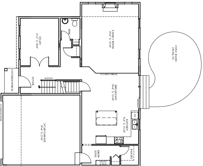
FIRST FLOOR PLAN 1,150 S.F.
