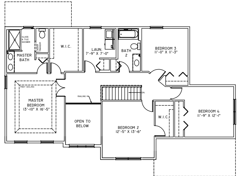
SECOND FLOOR PLAN 1,328 S.F.
