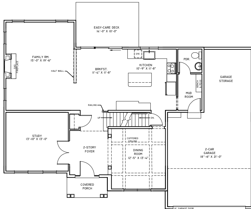
FIRST FLOOR PLAN 1,294 S.F.
