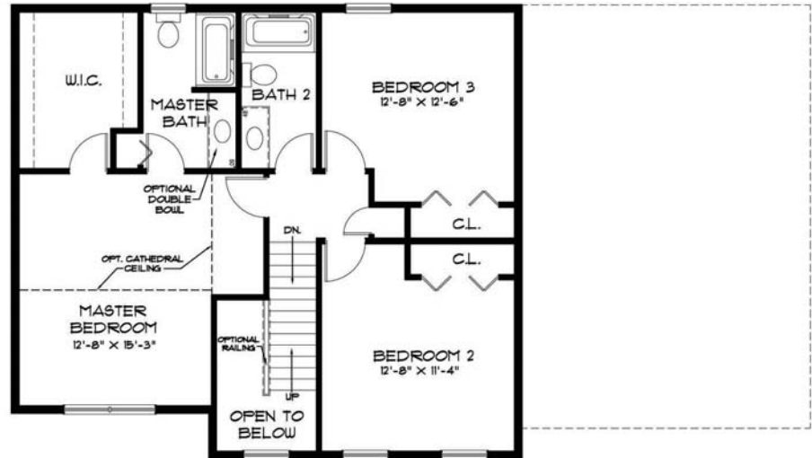
SECOND FLOOR 892 square feet
